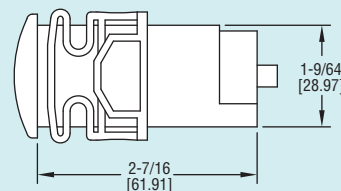
Panel Cutout 2-51/64 x 1-9/64 (71 x 29)
