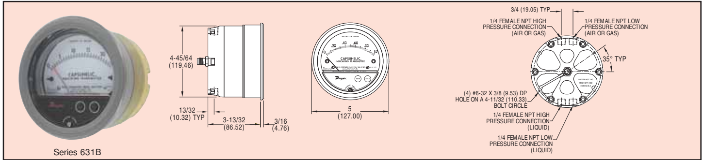
Series 631B
