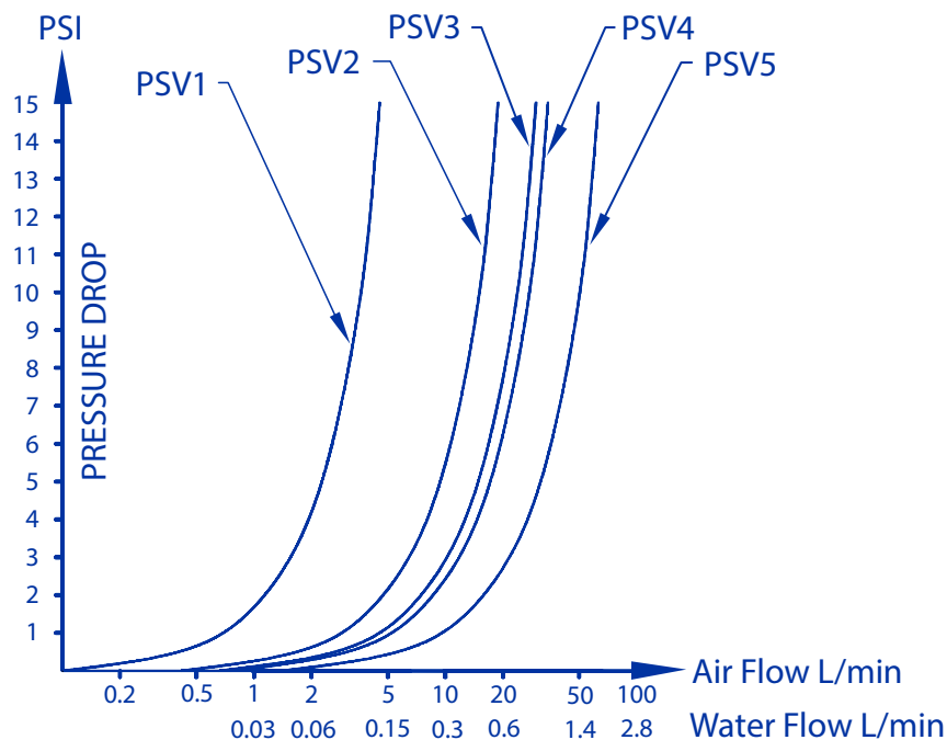
Pressure Drops Across PSV Valves
