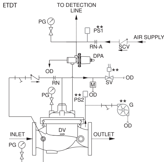
SCHEMATIC 12
