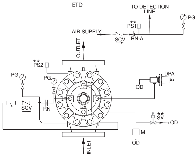
SCHEMATIC 2
