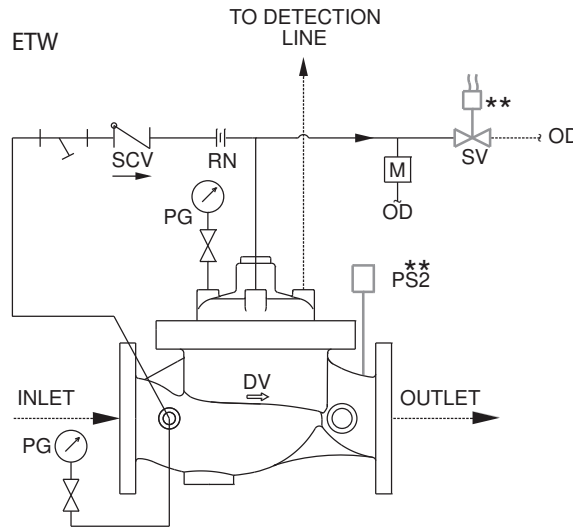
SCHMATIC 9
