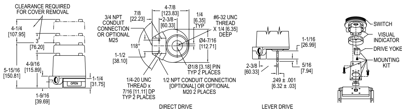
DIRECT DRIVE
