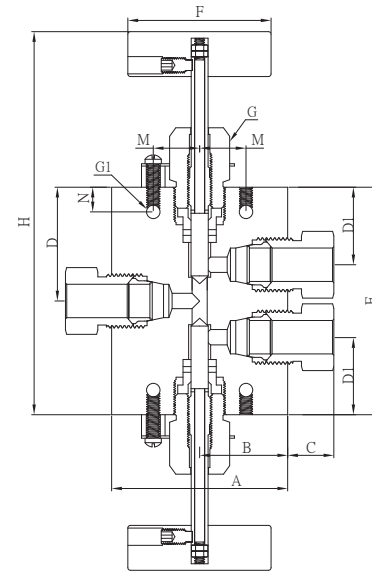
3-way/2 stem manifold
